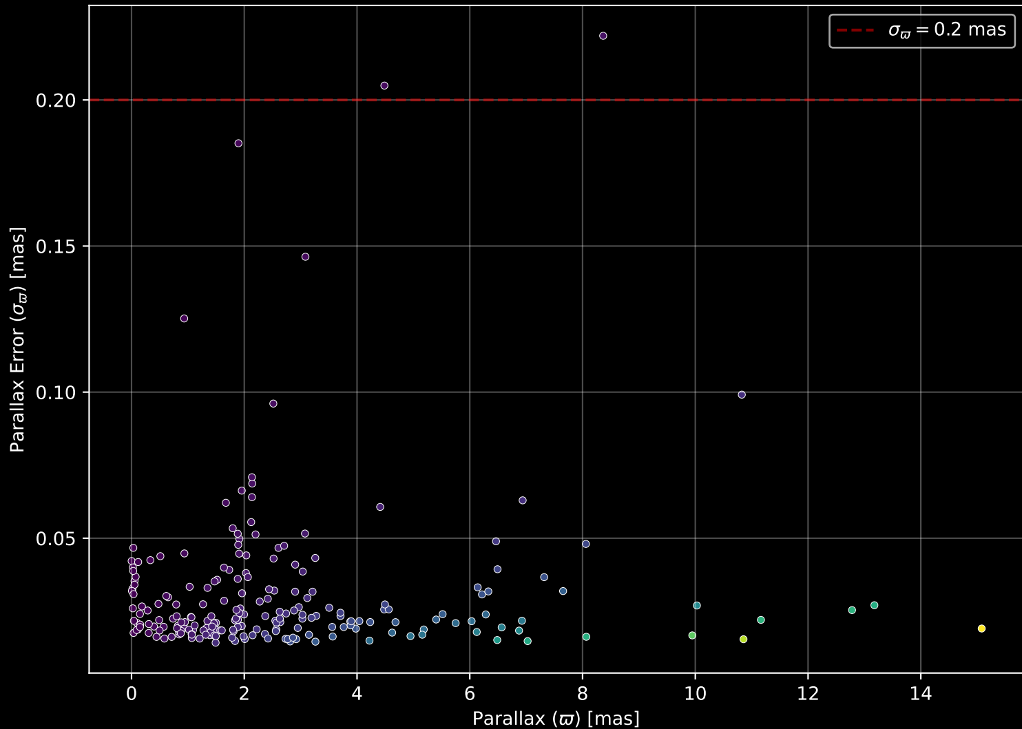
APOGEE DR17 Field: [209+73_btx] Parallax Quality (n= 216)
