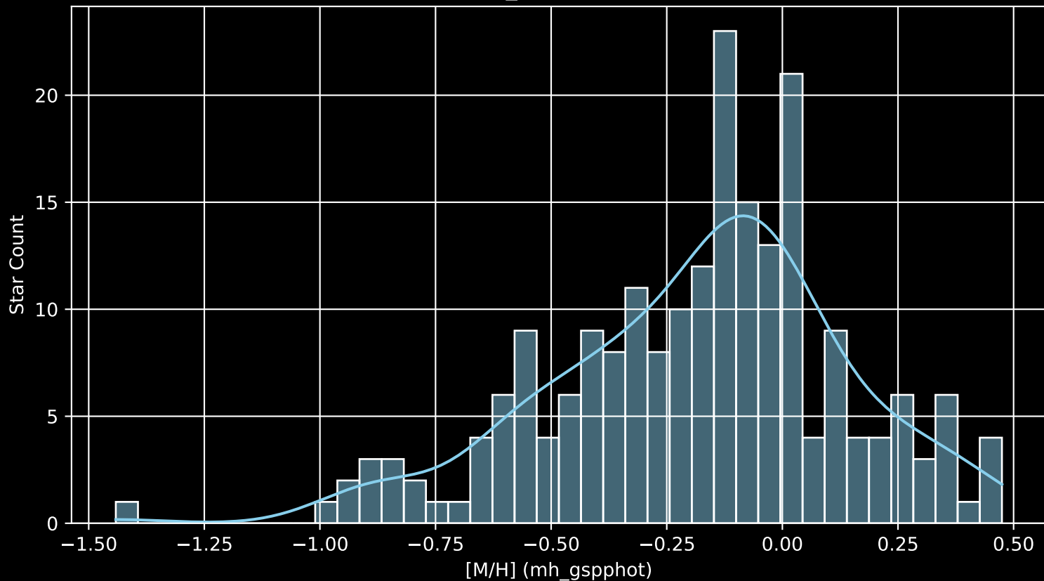
APOGEE DR17 Field: [209+73_btx [M/H] (mh_gspphot) (n= 214)
