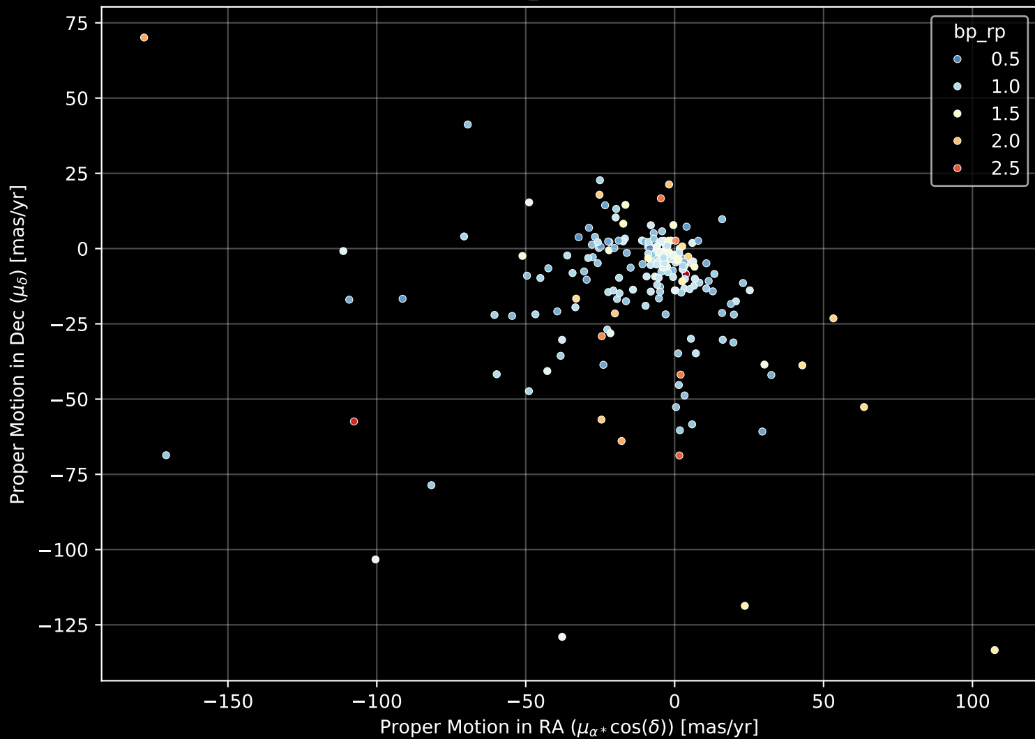
APOGEE DR17 Field: [209+73_btx] Proper Motion Diagram (n= 216)
