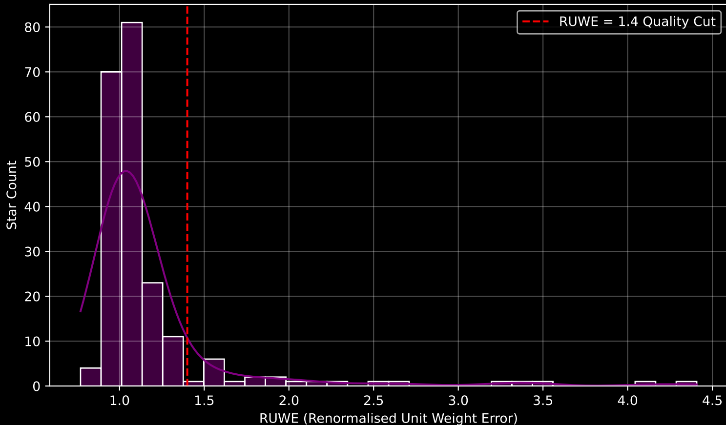
GAPOGEE DR17 Field [209+73_btx] RUWE Distribution (n= 211)
