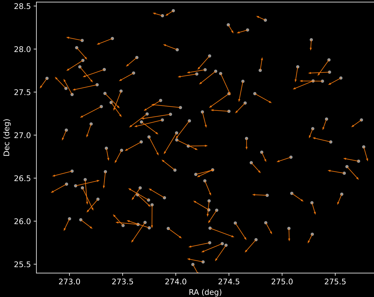
APOGEE DR17 Cluster 2 Proper Motion Vectors (n=110)
