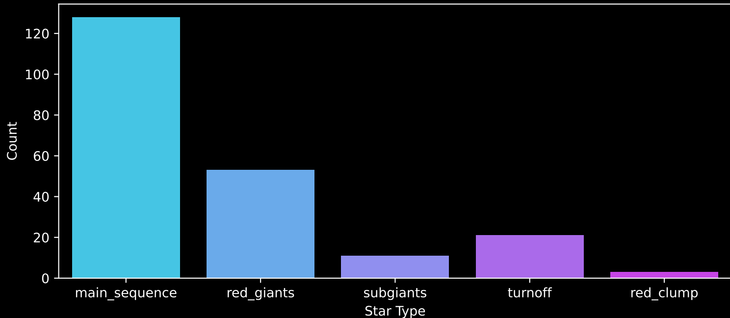
APOGEE DR17 Field: [209+73_btx] Count plot of Star Type
