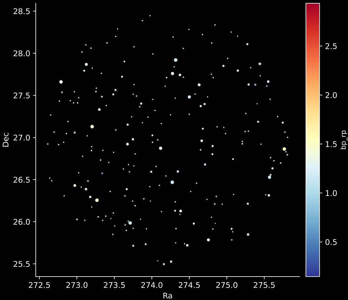
APOGEE DR17 Field: [209+73_btx] Stars: 216
